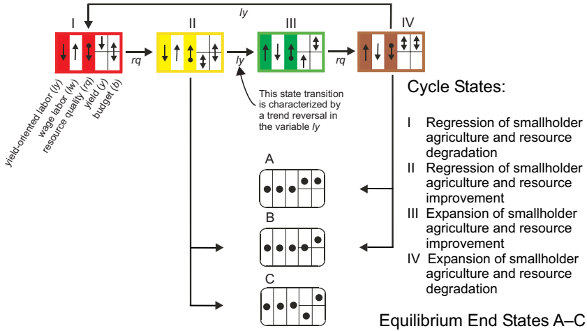
Figure 1.2 Symbolic dynamics of small agriculture in NE Brazil as a faithful projection to the five fundamental variables ly (yield-oriented labor), lw (wage-oriented labor), rq (resource quality), y (yield), and b (budget). The two sets of boxes represent cycle states (I–IV) and equilibrium end states (A–C), respectively, expressing magnitudes and trends of the fundamental variables by appropriate symbols. Dots indicate that the variable is constant over time, whereas trends are indicated by directed arrows. The crucial ly – rq trend combination is highlighted by color shading in the cycle state boxes. After Seitz et al., submitted.
