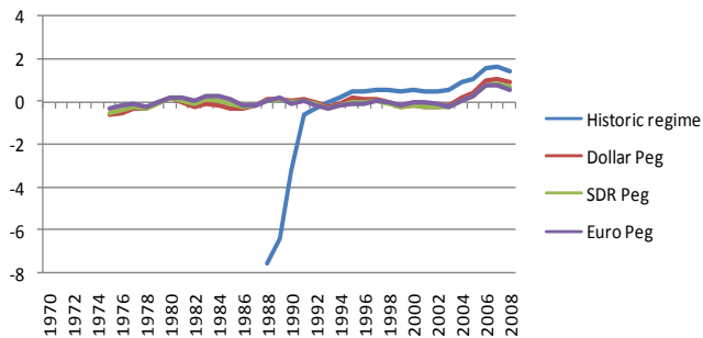
Peru, Nominal Export Price (in natural log, mean subtracted)
